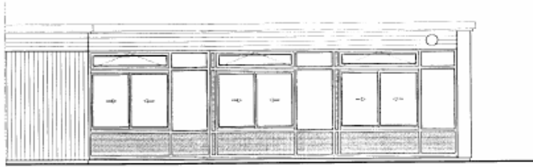
EXISTING WEST ELEVATION SCALE @ 1:50
